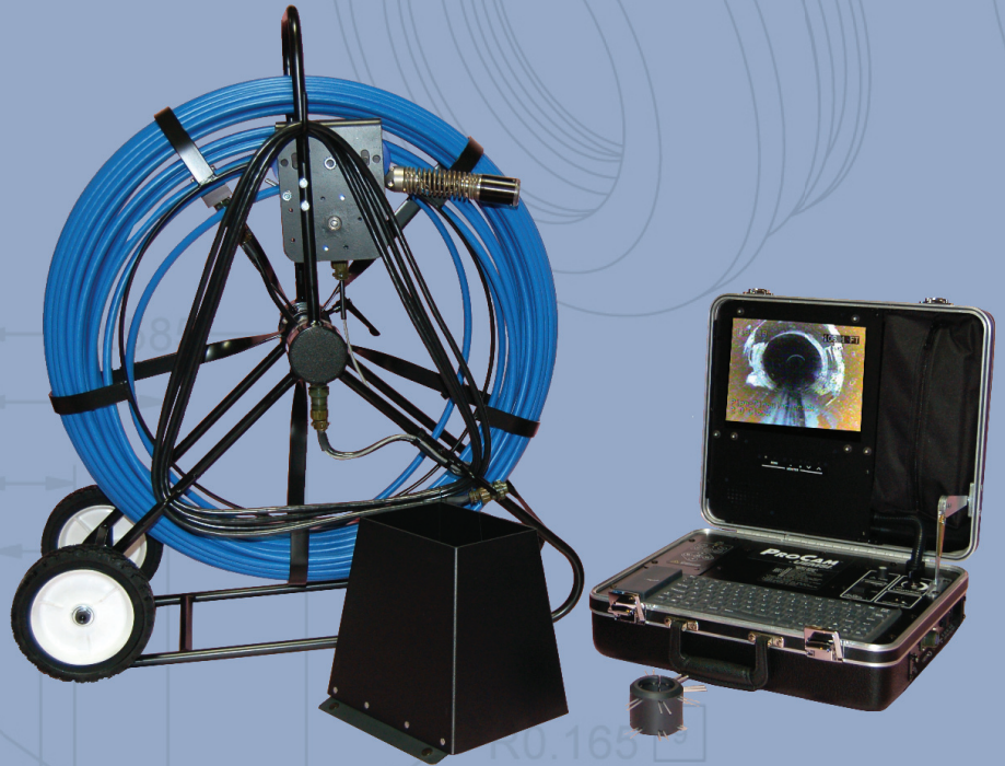
The ProCam DVR Ultra system is shown with standard features including reel w/ 200' of video push cable, CM-1 color camera head and Data Display I package w/ keyboard.
